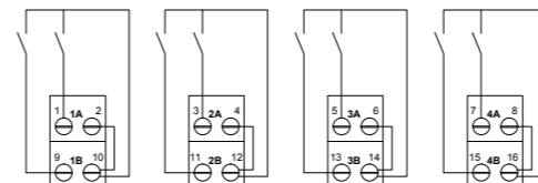
h Connection as a 4-fold binary input (connection of double pushbuttons dedicated to the control of dimmers or drives)
