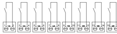
g Connection as a 8-channel binary input (connection of traditional switches or pushbuttons dedicated to the on/off switching of loads)
