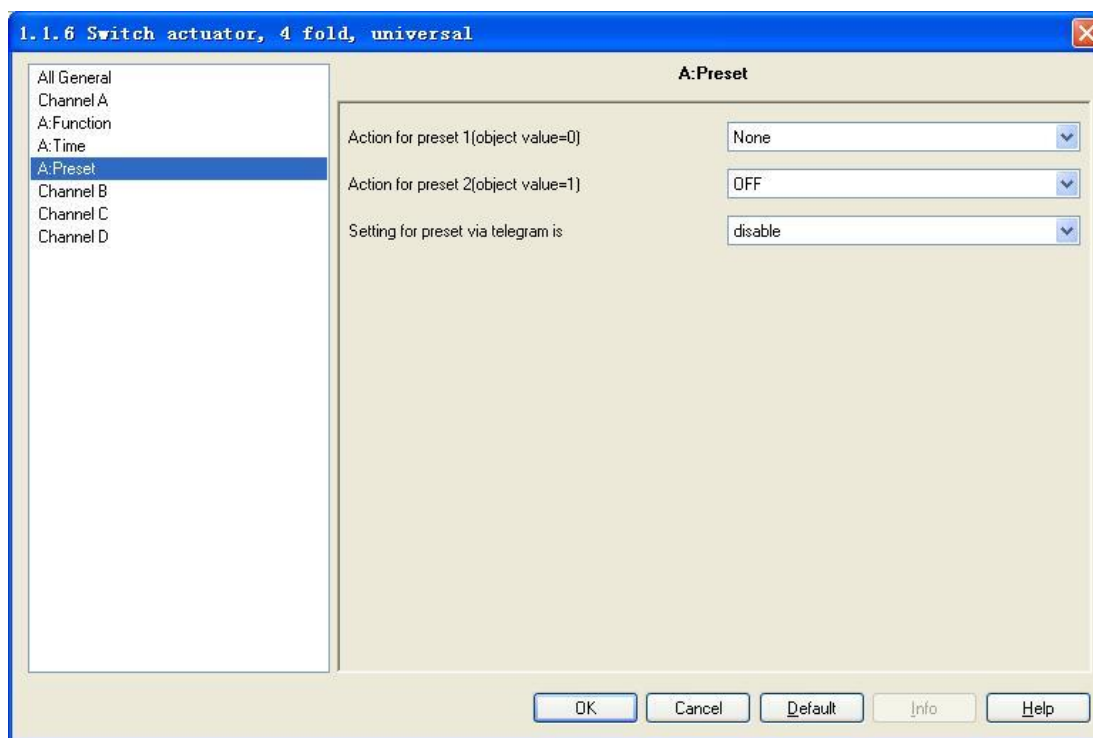
Fig.9 - Setup window "X: Preset"
