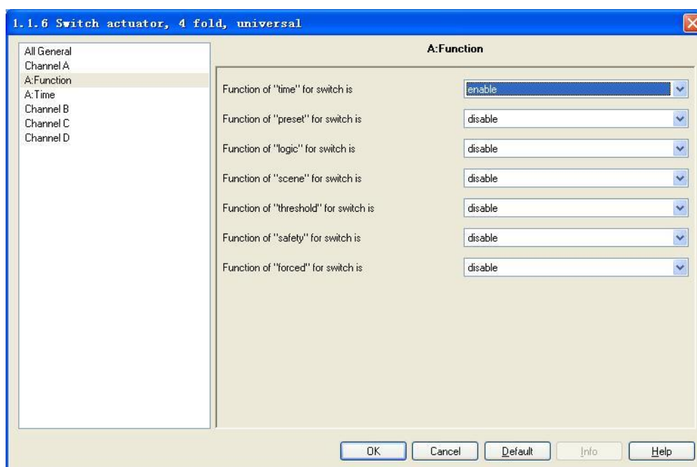
Fig.5 - Setup window "X: Function"
