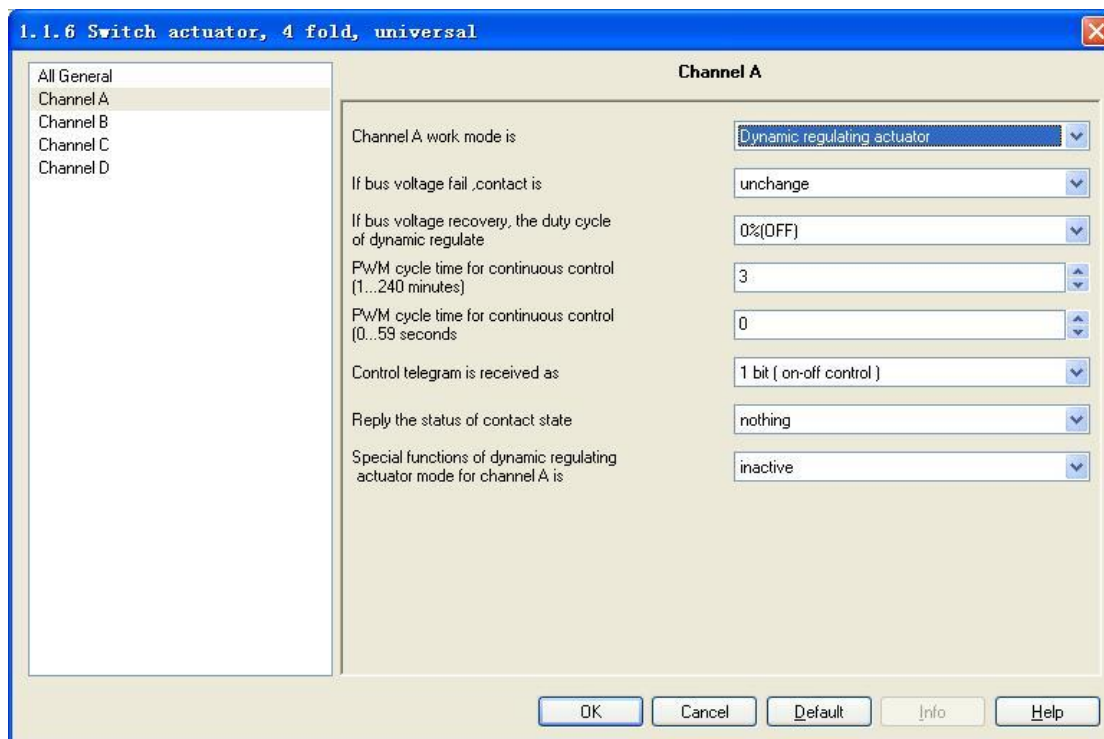
Fig.15 - Setup window “Channel: X - Dynamic regulating actuator”
