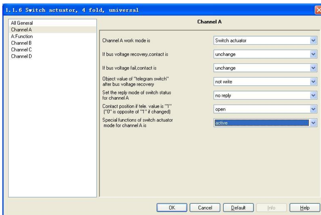
Fig.4 - Starting setup window “X: Function”
