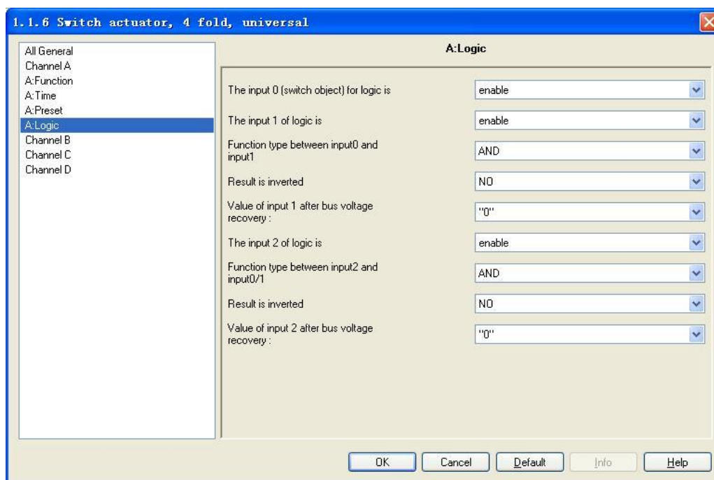
Fig.10 - Setup window "X: Logic"
