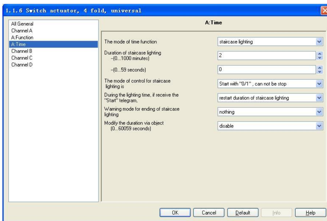
Fig. 7- Parameter window "X: Time-Staircase lighting"
