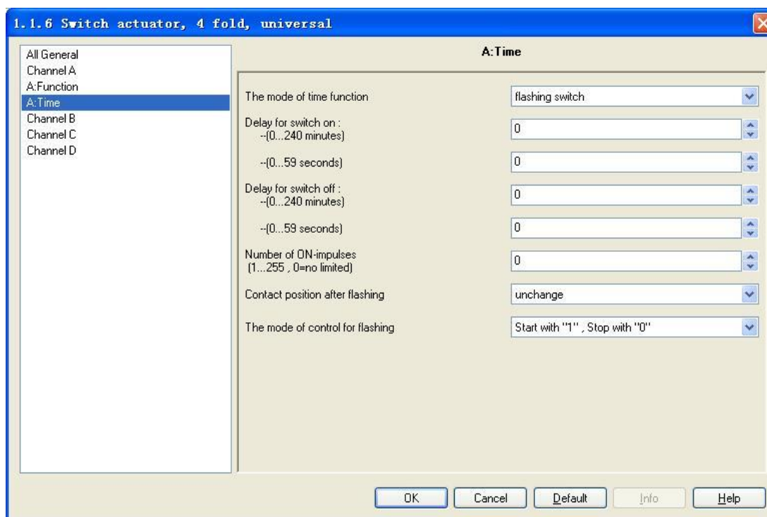
Fig.8 - Parameter window "X: Time-flashing switch"
